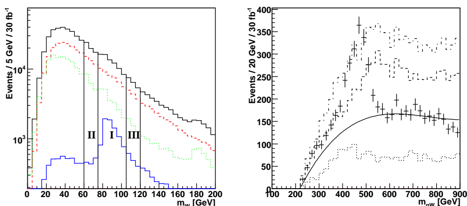
Figure 9: Left: Jet mass distribution for W candidates at the \alpha benchmark point following a cut on missing energy: \cancel{E}_T > 300 GeV. The SUSY signal (blue, solid), SUSY background (red, dashed) and SM background (green, dotted) contributions are also shown separately. Right: Invariant mass distribution of qW combinations for the \alpha benchmark point in the signal region (region I, points with error bars), in the sideband regions (region II dashed, region III dotted) and for the sum of sideband events (dashed dotted). Also shown is the fit to the sideband distribution (solid line), rescaled to the signal distribution.
