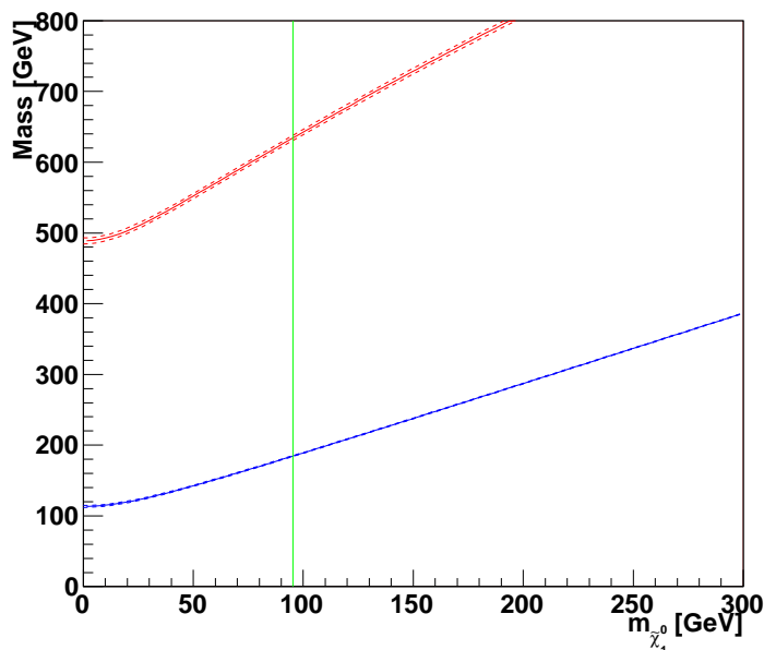
Figure 13: The squark (red) and \tilde{\chi}_1^\pm (blue) masses as a function of the \tilde{\chi}_1^0 mass for the \gamma benchmark point. The dashed lines show the 1\sigma statistical error bands. The vertical green line indicates the nominal \tilde{\chi}_1^0 mass.
