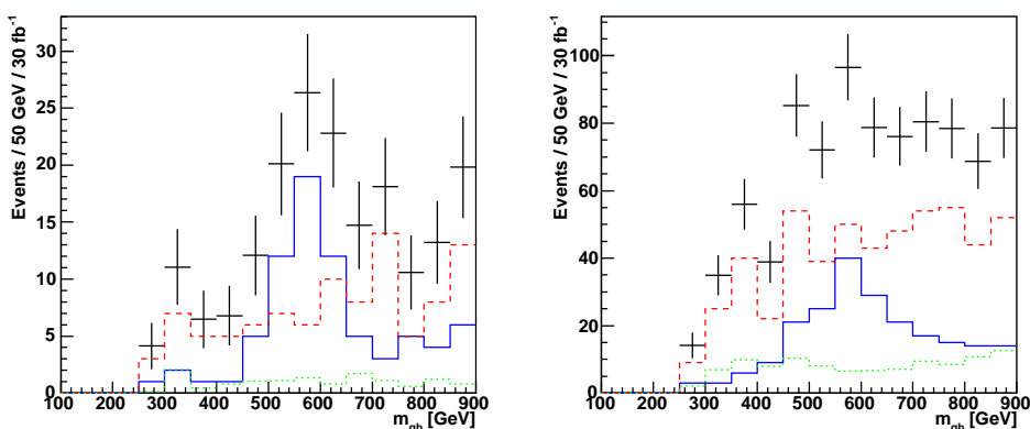
Figure 6: Figure 5f without the sub-jet scale cut (left) and without the jet-mass cut (right). See figure 4 and text for details.
