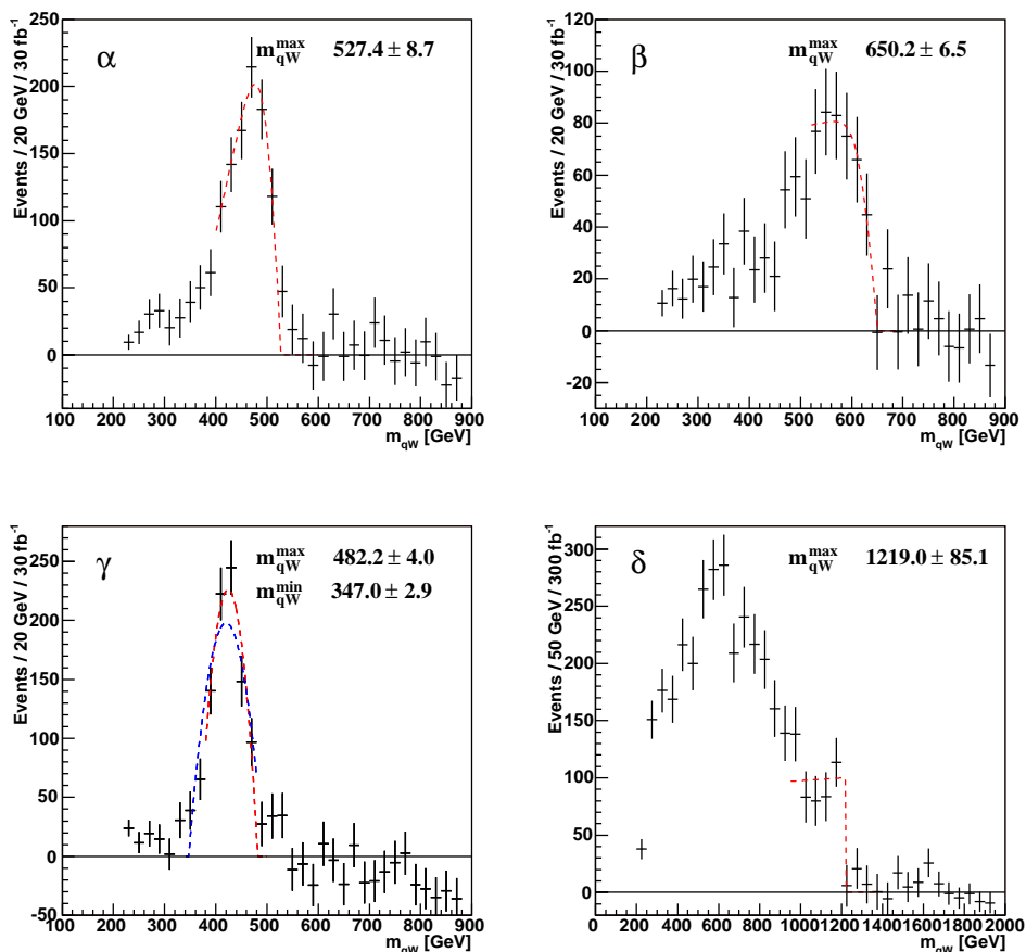
Figure 10: Invariant mass distribution of qW combinations at the four benchmark points, \alpha (top left), \beta (top right), \gamma (bottom left) and \delta (bottom right), after sideband subtraction. Also shown are fits to the upper edges of the distributions, and for \gamma also the clear lower edge.
