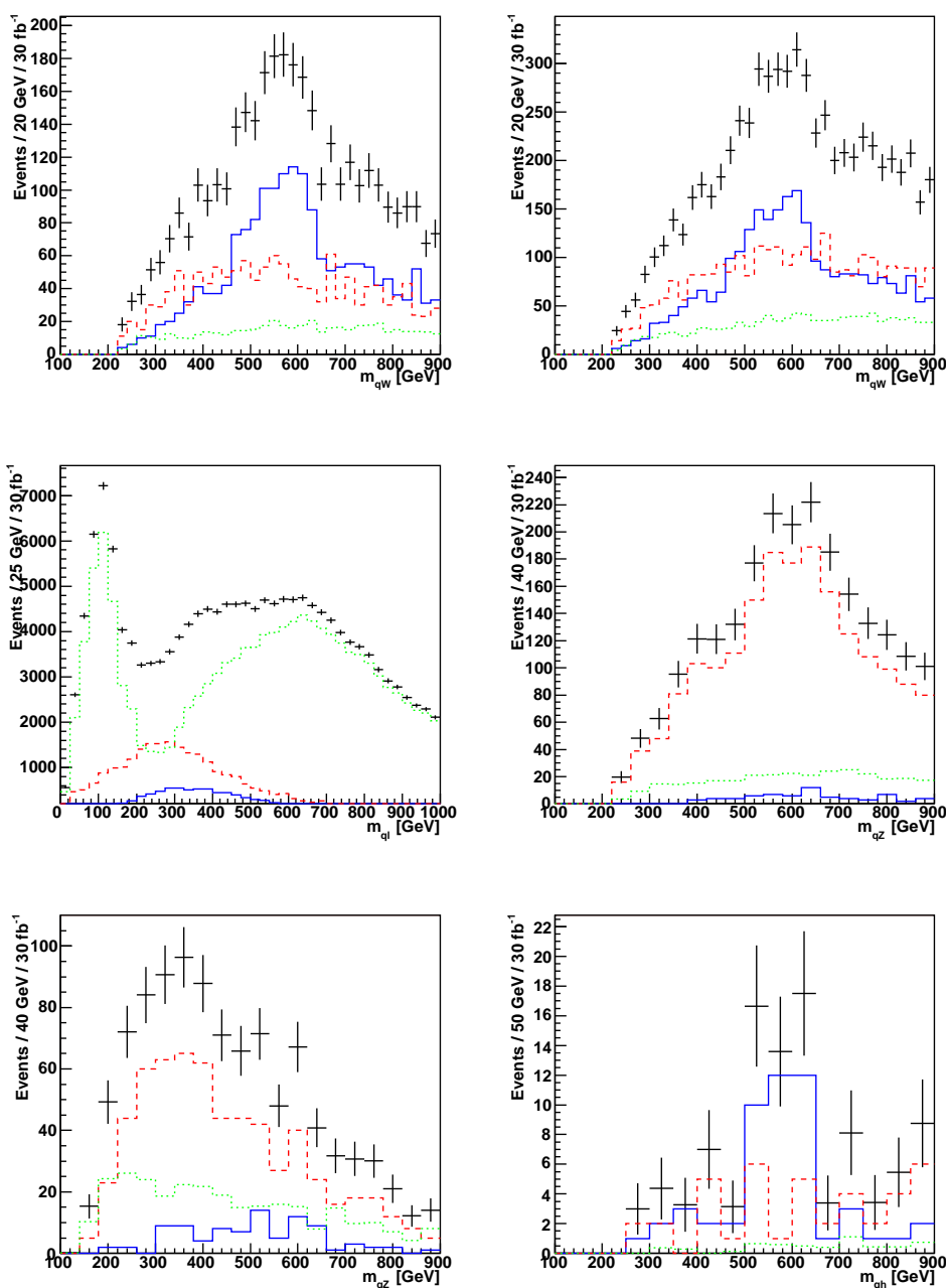
Figure 5: Various invariant mass distributions obtained in a simulation of events for SUSY benchmark scenario \beta . See figure 4 and text for details.
