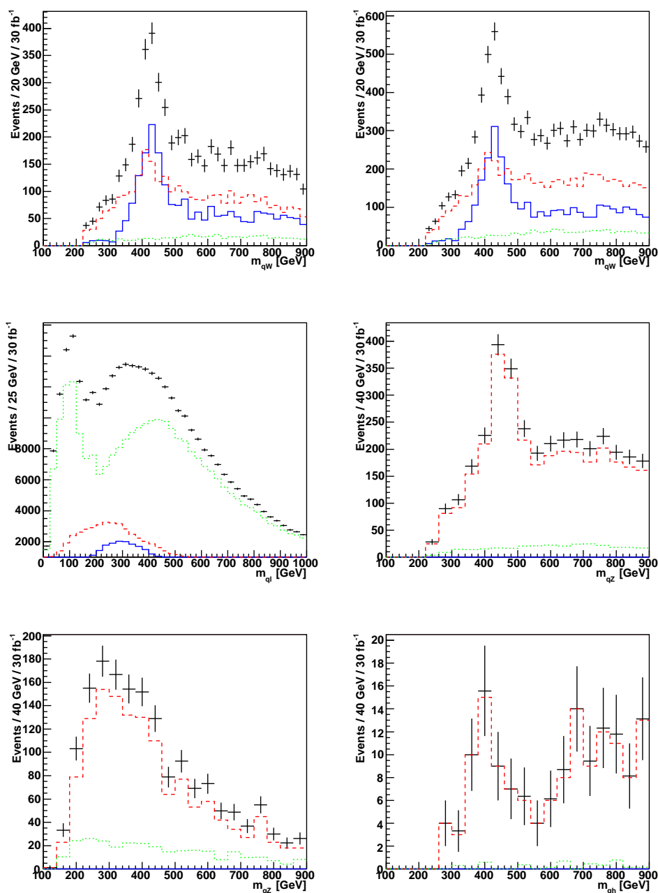
Figure 7: Various invariant mass distributions obtained in a simulation of events for SUSY benchmark scenario \gamma . See figure 4 and text for details.
