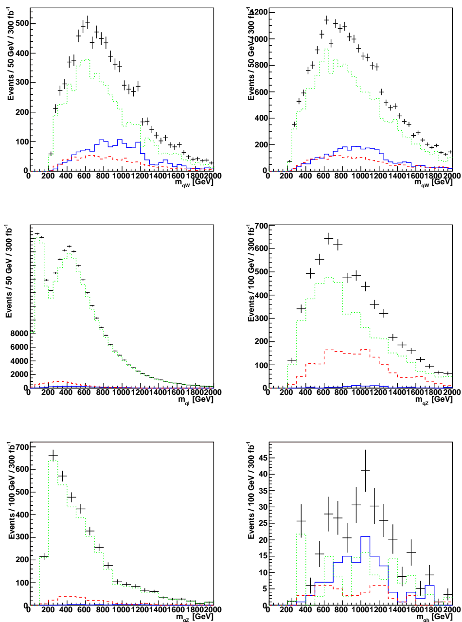
Figure 8: Various invariant mass distributions obtained in a simulation of events for SUSY benchmark scenario \delta . See figure 4 and text for details.
