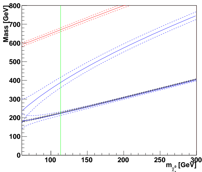
Figure 12: The squark (red), \tilde{\chi}_1^\pm (blue) and \tilde{\chi}_2^0 (black) masses as a function of the \tilde{\chi}_1^0 mass for the \alpha benchmark point. The dashed lines show the 1\sigma statistical error bands. The vertical green line indicates the nominal \tilde{\chi}_1^0 mass.
